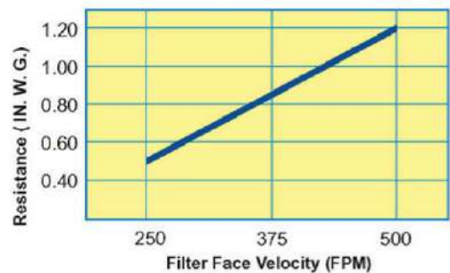
INITIAL RESISTANCE VS. FILTER FACE VELOCITY
